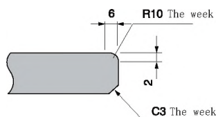
Chamfering shape Type A
